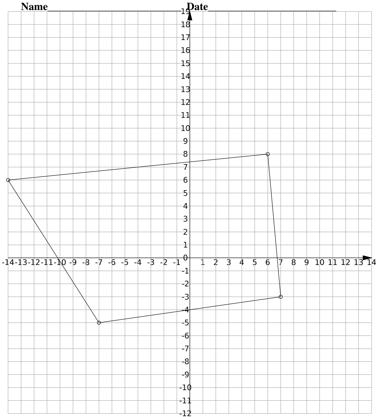
Shape: (-14,6), (6,8), (7,-3), (-7,-5)
